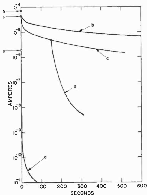
Fig. 9—Photocurrent decay in CdS at 18°C for various surface conditions. (a) 1 atmosphere dry air. (b) 3 \times 10^{-5} torr. (c) 3 \times 10^{-3} torr. (d) Effect of admitting dry air at 1 atmosphere during decay that commenced at 3 \times 10^{-3} torr [from Jour. Phys. Chem. Sol. , Vol. 25, p. 911 (1964)].
