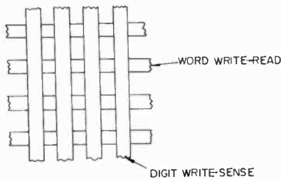
Fig. 15—Schematic of a word-organized memory array.
