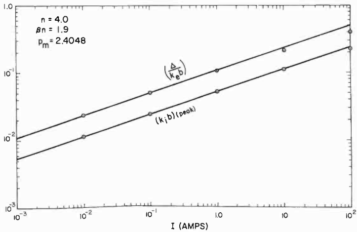
Fig. 7b—Peak gain and bandwidth versus average beam current, for n = 4.0 , \beta n = 1.9 , p_m = 2.4048 .
