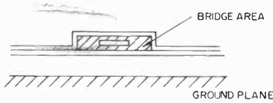
Fig. 2—Cross section of the bridge cell.
