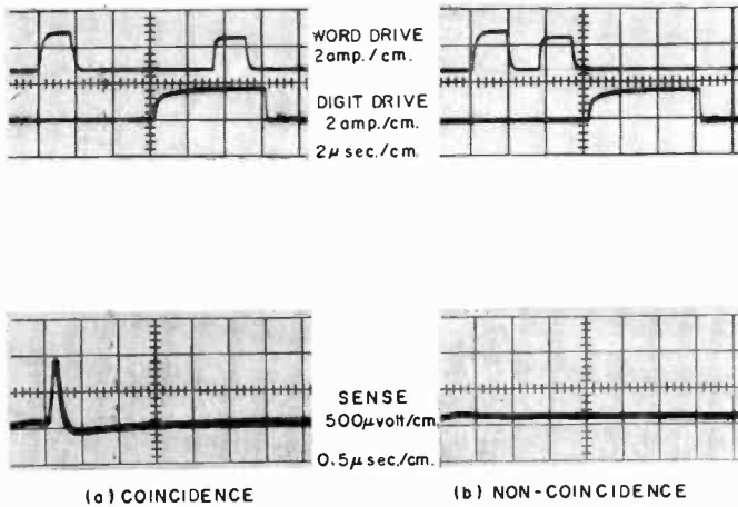
Fig. 8—Waveforms of word current, digit current, and sense voltage for both the coincident and the noncoincident conditions.
