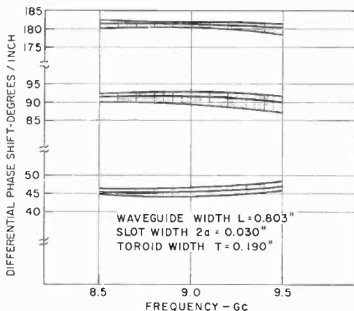
Fig. 14—Differential phase shift as a function of frequency. Heavy line indicates average of ten units; shaded portions indicate the spread.
