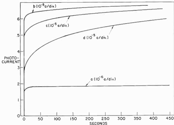
Fig. 12—Photoconductivity growth in CdS at 18°C for various surface conditions. (a) Growth in dry air at 1 atmosphere for all values of t_d between 1 and 30 minutes. (b), (c) and (d) represent the growth at 3 \times 10^{-5} torr for t_d = 1, 5, and 30 minutes, respectively [from Jour. Phys. Chem. Sol. , Vol. 25, p. 911 (1964)].
