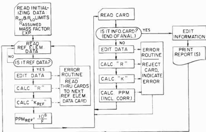
Fig. 4—Simplified flow chart of RCA 601 computer program for mass spectrographic analysis.
