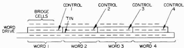
Fig. 18—Side view of one word line of a word-bit-organized array.
