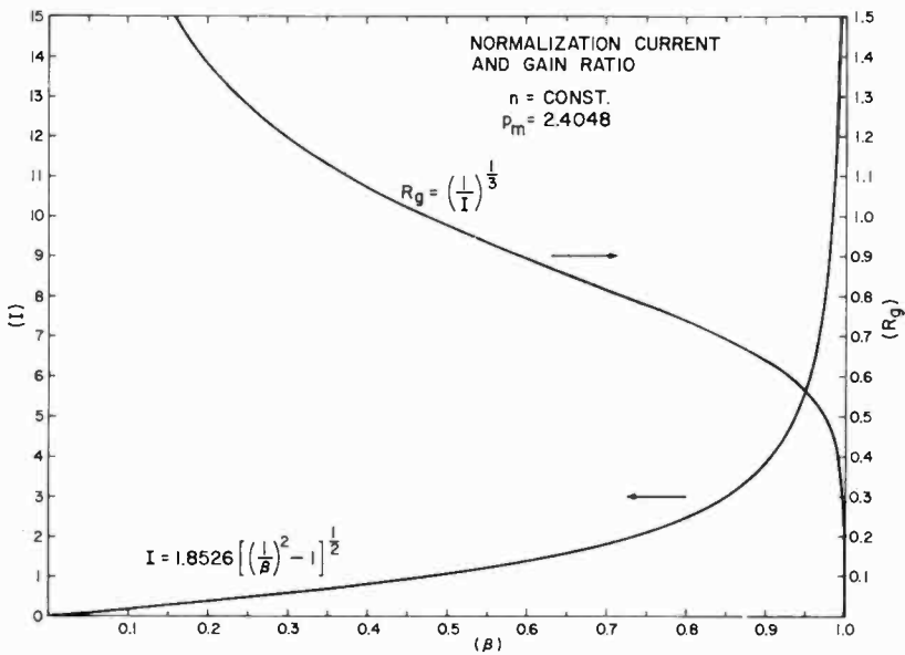
Fig. 8c—Current and gain normalizing factor versus \beta n for k_{p0} b = 2.0851 \times 10^{-2} .
