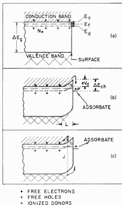
Fig. 1.—Model for spontaneous chemisorption on the surface of a wide-band-gap extrinsic semiconductor. (a) Energy-band configuration of an adsorbate-free surface; E_c is the bottom of the conduction band, E_f is the equilibrium Fermi level, E_d is the donor level, \Delta E_g is the band gap, N_+ is the ionized donor concentration. (b) Surface after chemisorption showing the Schottky-type surface barrier; V_d is the diffusion potential, \Delta E_{ch} is the energy of desorption, L is the thickness of the depletion layer, N_+ is again the ionized donor concentration in the depletion layer, \sigma is the concentration of chemisorbed ions. (c) Photodesorption when t_p < \tau_p ; J represents the optical generation of free electron-hole pairs.
