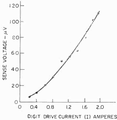
Fig. 11—Amplitude of the sense voltage as a function of the amplitude of the digit drive pulse.
