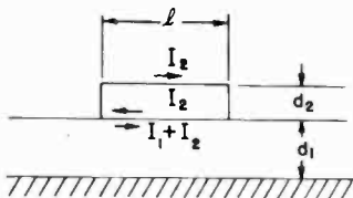
Fig. 4—Side view of the bridge cell.
